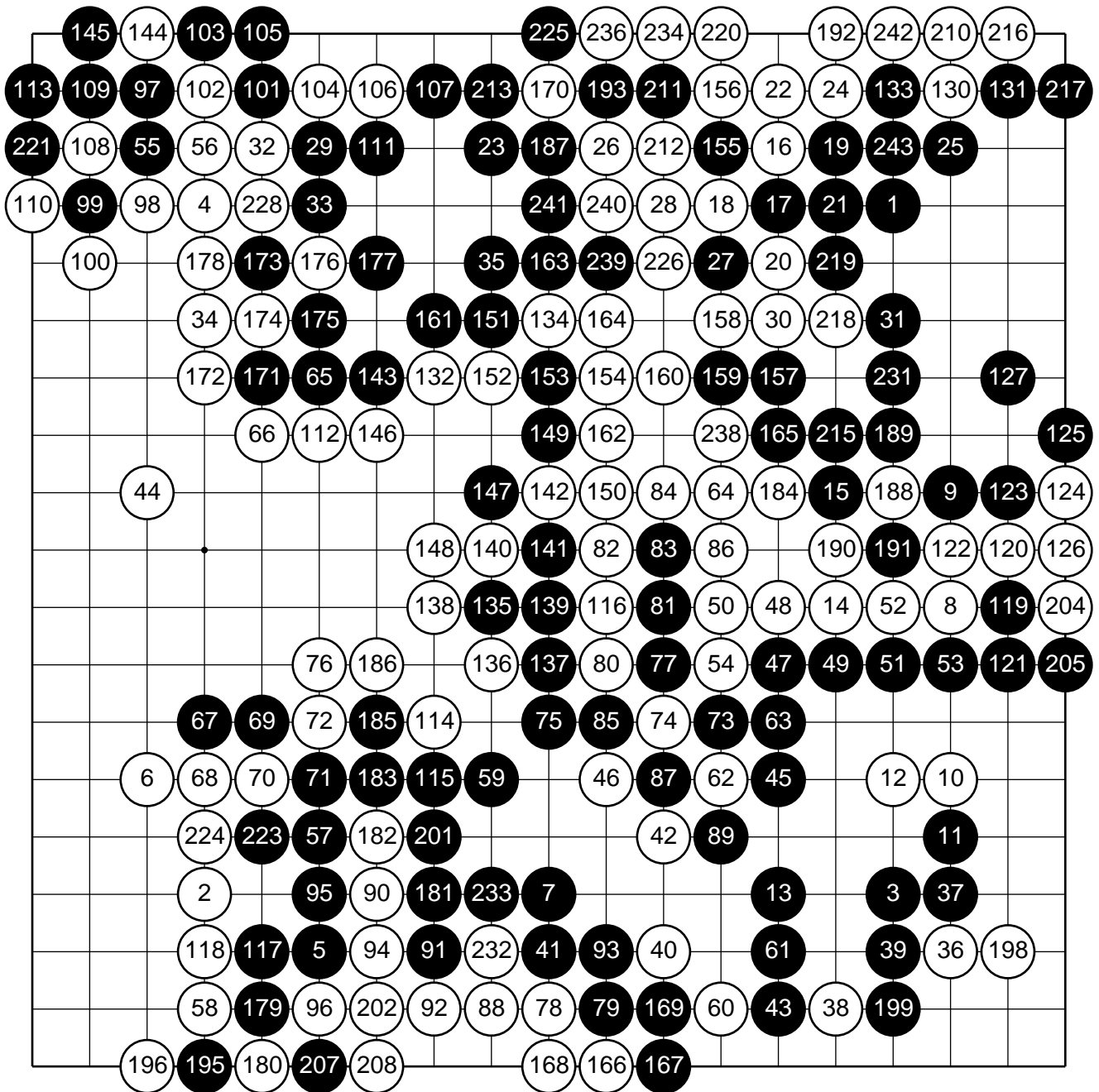
Game 1 - Figure 1 (1-244)
